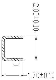
SEC:C-C
